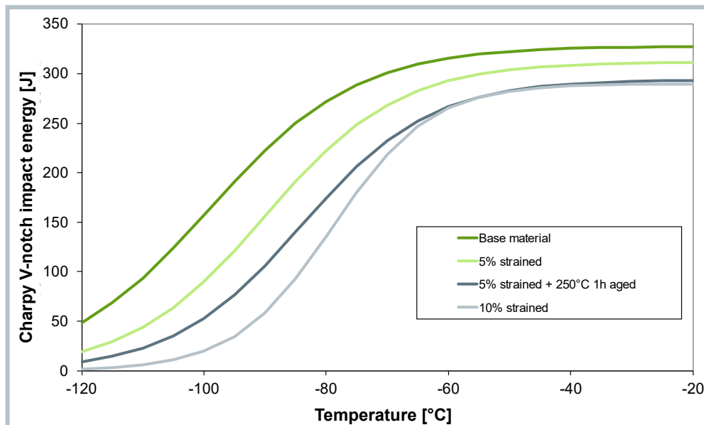
Example of the influence of cold deformation and ageing on the Charpy V-notch impact energy/temperature curve of DI-MC 355 T/S355ML (average curves, scatter not shown)
