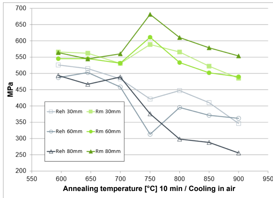
Plot of mechanical strength data for DI-MC 460/S460ML after laboratory annealing tests at various temperatures and 10 min. holding time
